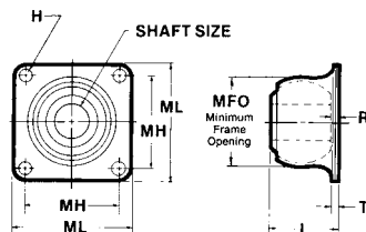
4-Bolt Side Flanges
