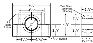
Custom Bearings
